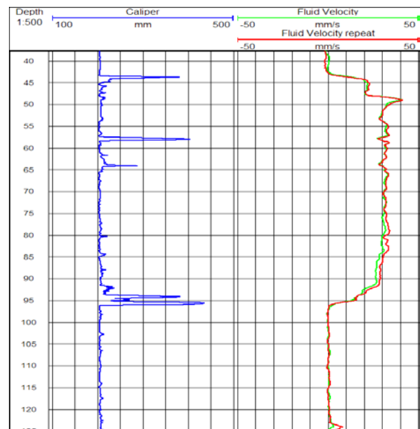
Impeller flowmeter log showing vertical watermovement between two issues
